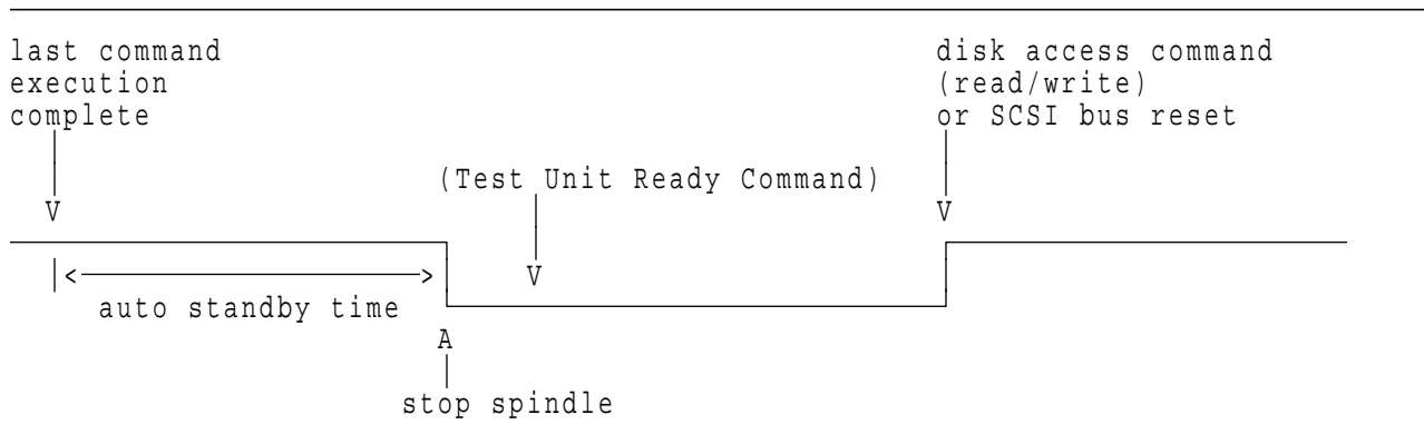
Figure 7-2. Power Save Function
