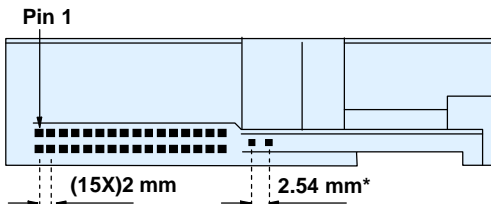
Jumper Pin locations (front view) - all models
