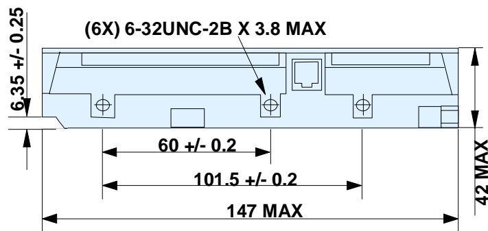
Location of side mounting holes.
