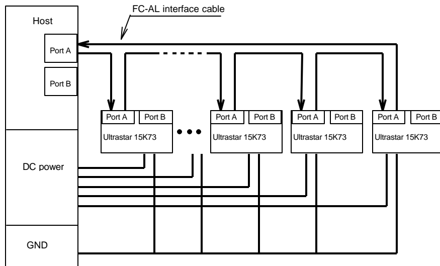
Figure 5.1 Cabling layout (Single Loop)
