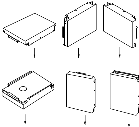
Figure 3.2 Shock test direction
