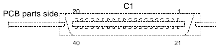
Figure 10.3 Connector view
