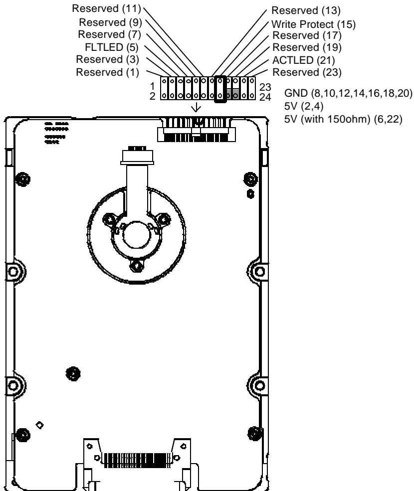
Figure 12.1 Jumper connector layout (SCA-2 Fibre Channel)
