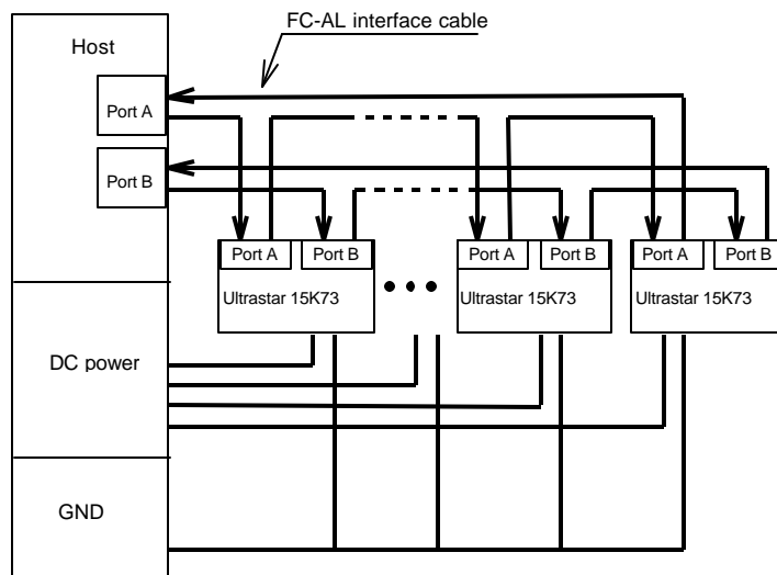
Figure 5.2 Cabling layout (Dual Loop)
